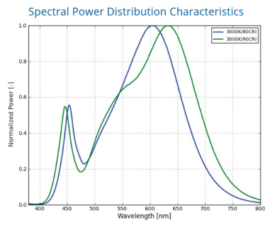
Figure 1. Typical normalized power vs. wavelength for LXZx-xxxx at test current, T_j=85^{\circ}\text{C} .
